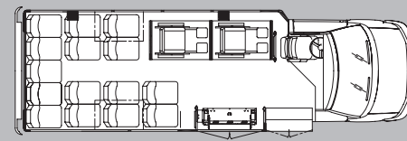
15 Passenger — Two Wheelchairs — Front Lift
