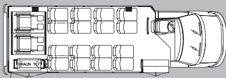
16 Passenger — Two Wheelchairs — Rear Lift
