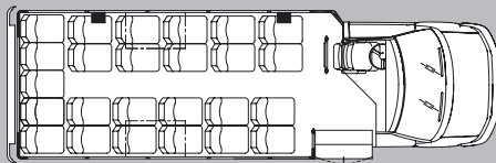
25 Passenger — Forward Facing Seating
